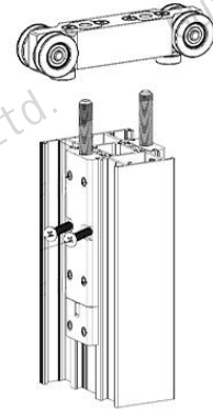
Hoist wheel
